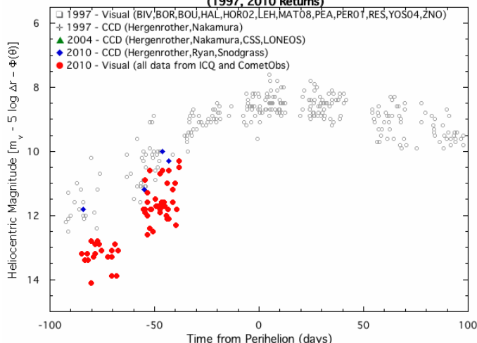
Heliocentric Lightcurve for Comet 103P/Hartley (1997, 2010 Returns)
