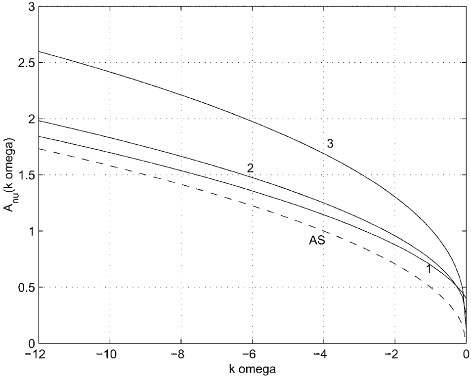
FIGURE 3 A_\nu(k\omega) for negative \nu : 1 - \nu = -1/2 , 2 - \nu = -1 , 3 - \nu = -3/2 , AS - lower bound 0.5\sqrt{-k\omega} .
