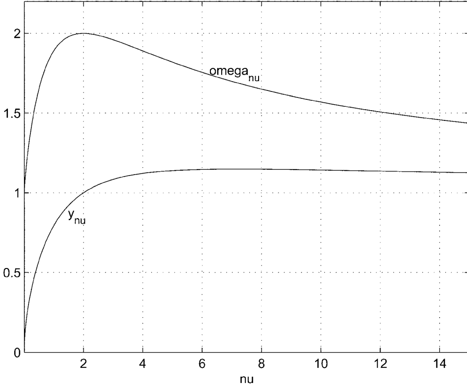
FIGURE 1 Parameters for the closed universe solution.
