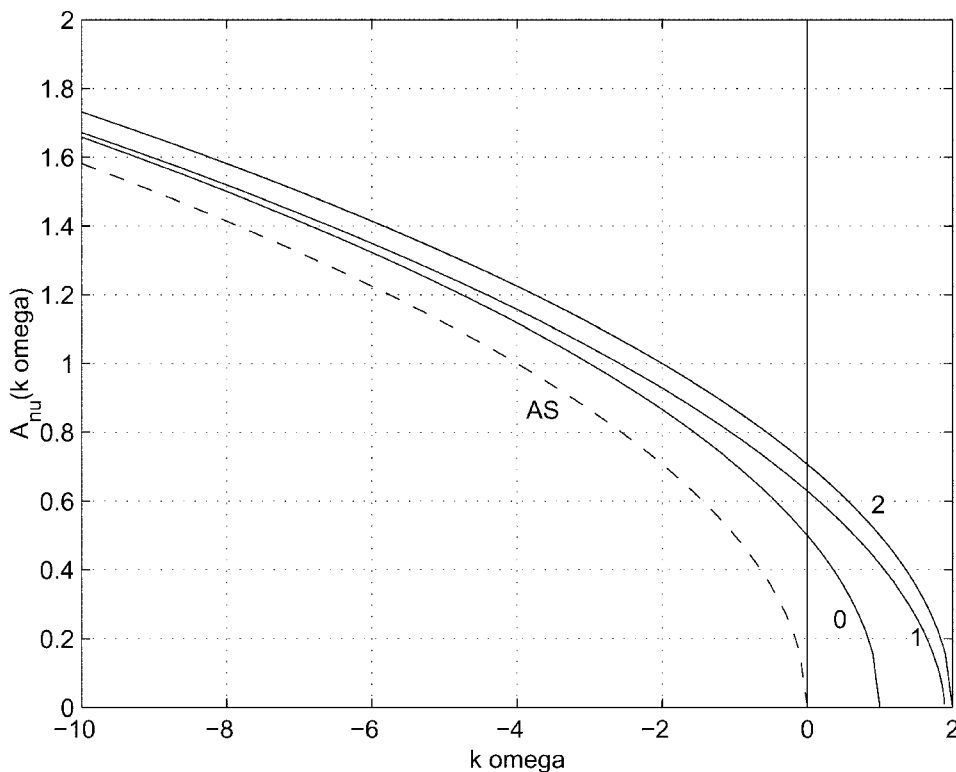
FIGURE 2 A_\nu(k\omega) for nonnegative \nu : 0 – \nu = 0 , 1 – \nu = 1 , 2 – \nu = 2 , AS – lower bound 0.5\sqrt{-k\omega} .
